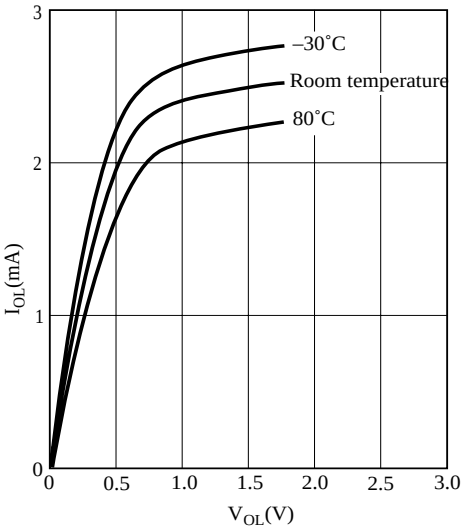
Figure 9.a. I_{OL} vs. V_{OL} Characteristic
