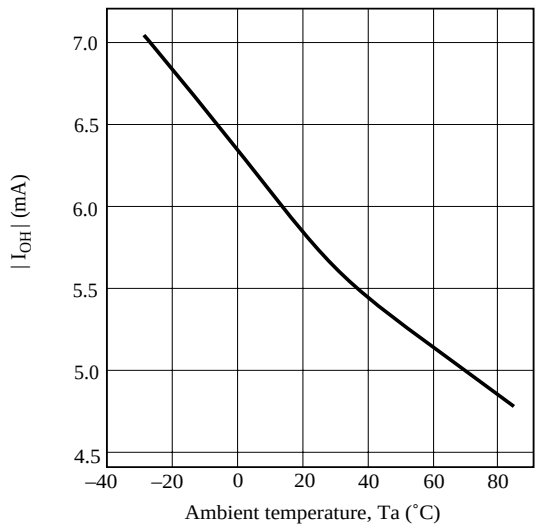
Figure 12.a. I OH vs. Temperature Characteristic
